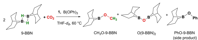
Scheme 3. CO 2 hydroboration in the presence of 1 and 9-BBN.
