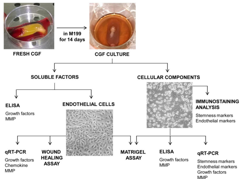
Figure 1. Experimental design.
