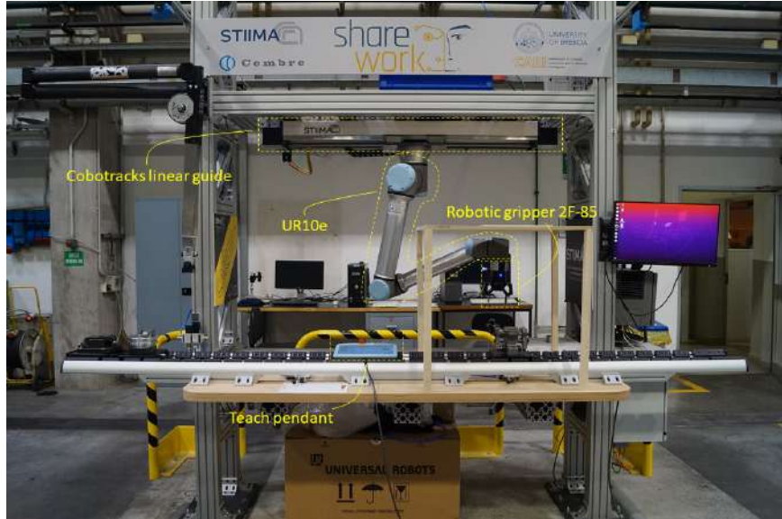
Figure 8. Experiment setup.
