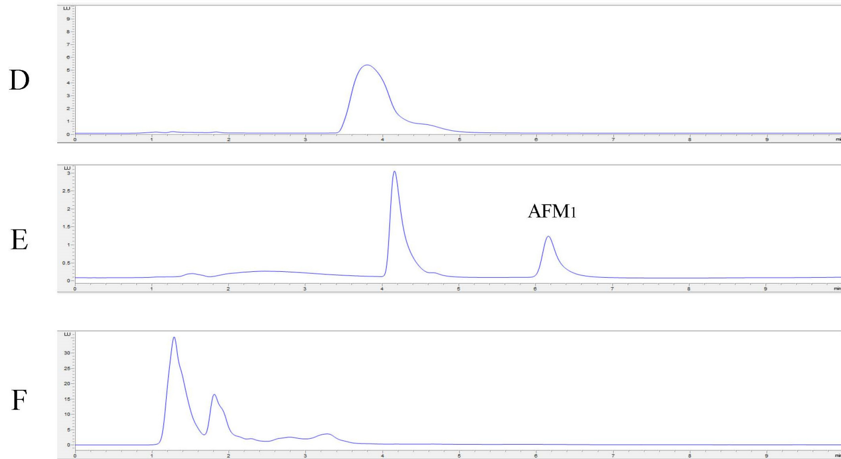
Figure 3. Examples of HPLC chromatograms of AFB 1 ( A —negative control, B —positive control, C —sample after degradation by Lac2) and AFM 1 ( D —negative control, E —positive control, F —sample after degradation by Lac2).
