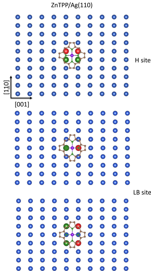
Fig. 12 Schematic representation of the ^{S_H}Ag_{110}^{nn} (upper panel), ^{S_{LB}}Ag_{110}^{nn} (middle panel), and ^{S_{LB}}Ag_{110}^{nn} (bottom panel) 5s AOs SALCs transforming as the ir b in the local C_2 symmetry of the Ag(110) bulk-terminate surface superimposed to the optimized ^{pmc}ZnTPP placed at 2.8 \text{ \AA} above the substrate and oriented with Ni-N^{Py} bonds aligned along the [1\bar{1}0] and [001] directions. Only Ag(110) topmost layer atoms are displayed for clarity. Large spheres represent ^{S}Ag^{nn} and ^{S}Ag^{nnn} 5s AOs, while different colors account for their different phases.
