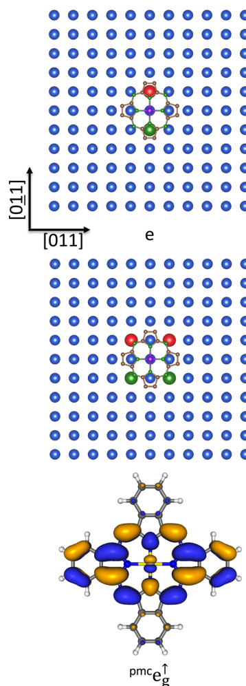
Fig. 7 Schematic representation of one component of the 5d_{100}^{6s} (upper panel), 5d_{100}^{6s} (middle panel) SALC of symmetry e on the Au(100) bulk-terminated surface superimposed to the optimized {}^{\text{pmc}}\text{CoPc} placed at 3.0 Å above the substrate and oriented with Co–N Py bonds aligned to the [011] and [011] directions. Only Au(100) topmost layer atoms are displayed for clarity. Large spheres represent 5d_{100}^{6s} and 5d_{100}^{6s} AOs, while different colors account for their different phases. 3D CP of one component of the e_g^{\text{pmc}}e_g^{\uparrow} SOs (lower panel). Displayed isosurfaces correspond to \pm 0.02 e^{\frac{1}{2}} \text{Å}^{-3/2} values.
