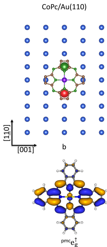
Fig. 6 Schematic representation of the 5d_{110}^{6s} SALC of symmetry b on the Au(110) bulk-terminated surfaces superimposed to the optimized {}^{\text{pmc}}\text{CoPc} placed at 3.0 Å above the substrate and oriented with Co–N Py bonds aligned along the [110] and [001] directions. Only Au(110) topmost layer atoms are displayed for clarity. Large spheres represent 5d_{110}^{6s} AOs, while different colors account for their different phases (upper panel). 3D CP of one component of the e_g^{\text{pmc}}e_g^{\uparrow} SOs (lower panel). Displayed isosurfaces correspond to \pm 0.02 e^{\frac{1}{2}} \text{Å}^{-3/2} values.
