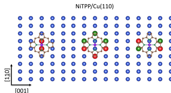
Fig. 11 Schematic representation of the ^{\text{S}}_{\text{SB}}\text{Cu}_{110}^{\text{II}} 4s AOs SALC of symmetry a in the local C_2 symmetry of the Cu(110) bulk-terminate surface (left panel), ^{\text{S}}_{\text{SB}}\text{Cu}_{110}^{\text{II}} 4s AOs SALC of symmetry b in the local C_2 symmetry of the Cu(110) bulk-terminate surface (central panel), ^{\text{S}}_{\text{SB}}\text{Cu}_{110}^{\text{II}} 4s AOs SALC of symmetry a in the local C_2 symmetry of the Cu(110) bulk-terminate surface superimposed to the optimized ^{\text{pmc}}\text{NiTPP} placed at 2 Å above the substrate and oriented with Ni–N Py bonds aligned along the [110] and [001] directions. Only Cu(110) topmost layer atoms are displayed for clarity. Large spheres represent ^{\text{S}}_{\text{SB}}\text{Cu}_{110}^{\text{II}} and ^{\text{S}}_{\text{SB}}\text{Cu}_{110}^{\text{II}} 4s AOs, while different colors account for their different phases.
