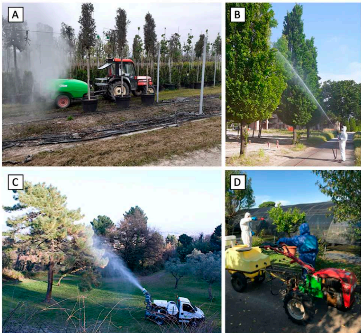
Figure 1. Conventional methods for pesticide distribution used in the ornamental plant sector. (A) A trailed agricultural atomiser (air-blast sprayer) used for potted or in soil trees or big shrubs; (B) a long-range spray gun commonly used for single trees or shrubs; (C) a centrifugal fan with long-range and wide-angle spray treatments commonly used for high trees; (D) a boom sprayer used for intra- and inter-row treatments, both in greenhouses and open-fields.
