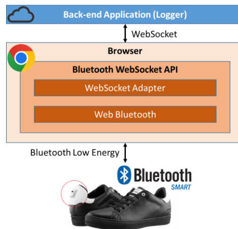
Figure 3. The Web App collects data from BLE shoes and sends it to the remote logger
