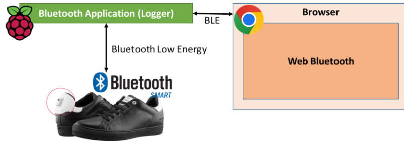
Figure 5. The Web App connects to the logger service which, in turn, collects the data directly from the BLE shoes
