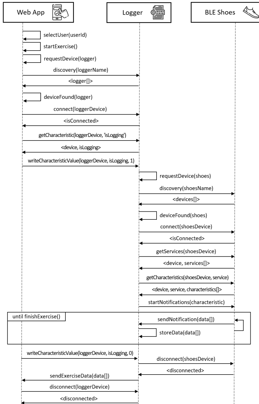
Figure 6. Sequence diagram of the interaction among the devices in the scenario 2
