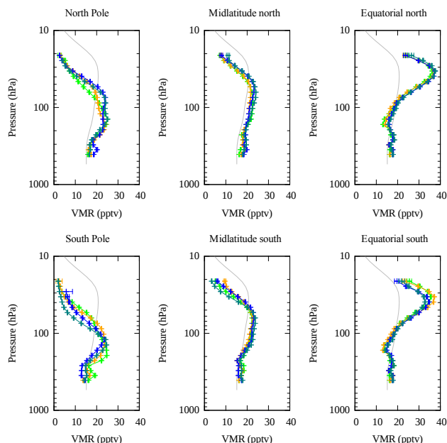
Figure 5. Average phosgene VMR profiles for DJF (green), MAM (orange), JJA (blue) and SON (light blue). Averages are calculated for North Pole (90–65° N, top left), midlatitude north (65–20° N, top centre), equatorial north (20–0°, top right), South Pole (65–90° S, bottom left), midlatitude south (20–65° S, bottom centre) and equatorial south (0–20° S, bottom right). We also report the a priori profile (solid grey) based on the existing climatology. This profile does not reproduce the observed geographical variability.
