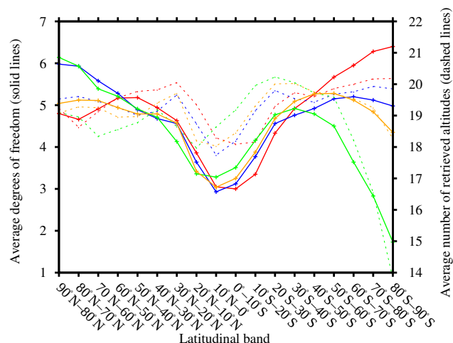
Figure 4. Average phosgene degrees of freedom (DOF, solid lines) and average of retrieved altitudes (dashed lines) for DJF (red), MAM (blue), JJA (green) and SON (orange). Averages are calculated for 10° latitude bins.
