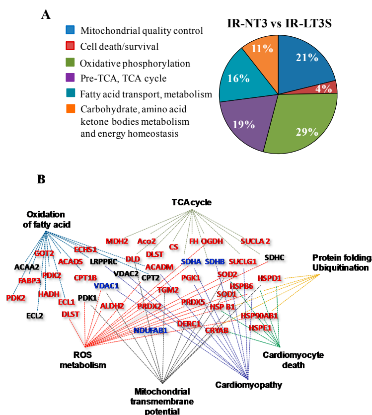
Figure 2. Mitochondrial proteomic analysis obtained at 72 h post IR. (A) Pie chart showing percentage of differentially expressed proteins grouped according to their function in IR-NT3 vs. IR-LT3S; and (B) clustering of differentially expressed proteins in IR-LT3S vs. IR-NT3 generated by IPA software. Networks related to diseases, functions and canonical pathways were generated based on the information stored in IPA Knowledge base. Network nodes are named by correspondent Gene Codes. The color assigned to node name indicate the level of proteins expression: red for up-regulated, blue for down-regulated and black for no change in IR-NT3 vs. IR-LT3S respectively. Gene acronyms are listed in the abbreviation list.
