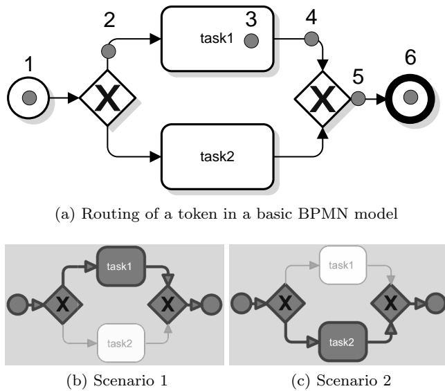
Fig. 4: Simple simulation scenarios of a basic BPMN model
