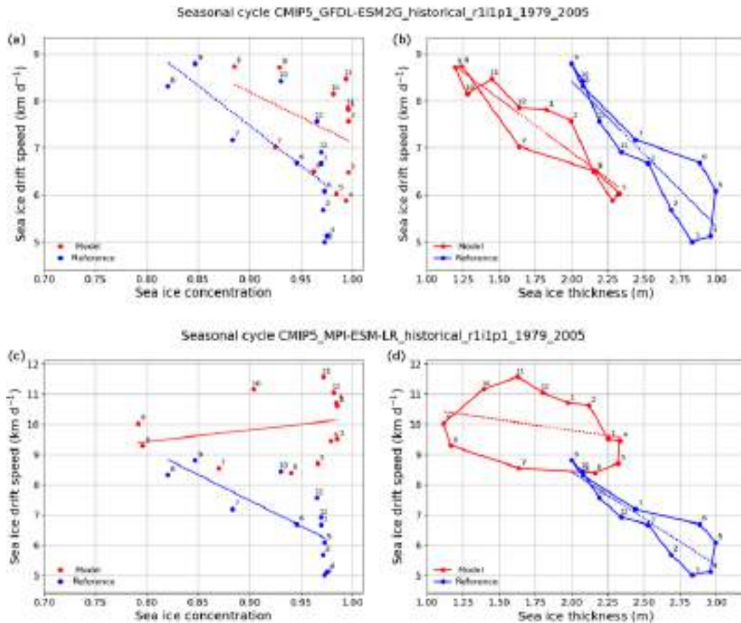
Figure 32. Scatter plots of modelled (red) and observed (blue) monthly mean sea ice drift speed against sea ice concentration (a, c) and sea ice thickness (b, d) temporally averaged over the period 1979–2005 and spatially averaged over the SCICEX box. Panels (a, b) show results from the GFDL-ESM2G model and (c, d) show results from the MPI-ESM-LR model (CMIP5 historical runs). Observations/reanalysis are shown in all panels (IABP for drift speed, OSI-450 for concentration, and PIOMAS for thickness). Numbers denote months. Dotted lines show linear regressions. This figure was produced in a similar way to Fig. 4 of Docquier et al. (2017) with recipe_sea_ice_drift.yml ; see details in Sect. 3.3.4.
