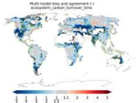
Figure 37. Global distribution of the biases in the multi-model ensemble ecosystem turnover time of carbon (years) and the multi-model agreement in CMIP5 models. The bias is calculated as the ratio between multi-model ensemble and observation-based estimate (Carvalhais et al., 2014). The stippling indicates the regions where only two or fewer models (out of 10) are within the range of observational uncertainties (5th and 95th percentiles). Produced with recipe_carvalhais2014nat.yml ; see details in Sect. 3.5.2.
