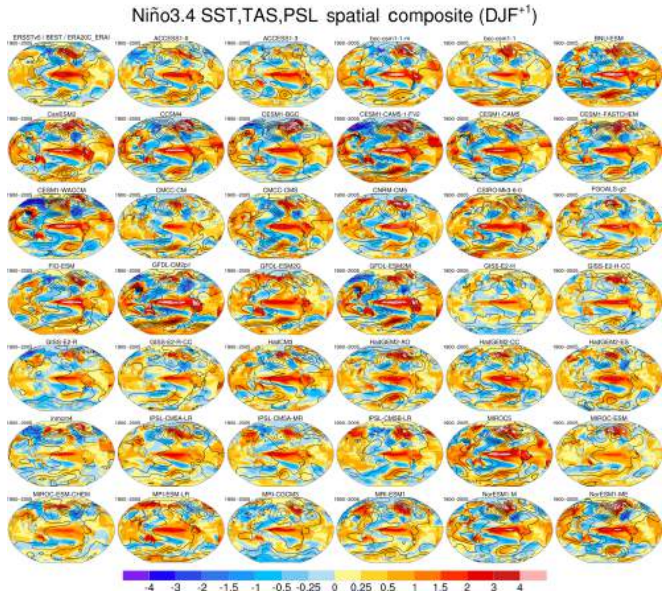
Figure 13. Global ENSO teleconnections during the peak phase (December–February) as simulated by 41 CMIP5 models (individual panels labelled by model name) and observations (first row, upper left panel) for the historical period (1900–2005 for models and 1920–2017 for observations). These patterns are based on composite differences between all El Niño events and all La Niña events (using a \pm 1 standard deviation threshold of the Niño 3.4 SST Index) occurring in the period of record. Colour shading denotes SST and terrestrial TREFHT (surface air temperature at reference height) ( ^{\circ}\text{C} ), and contours denote sea level pressure (psl); contour interval of 2 hPa, with negative values dashed. The period of record is given in the upper left of each panel. Observational composites use ERSSTv5 for SST, BEST for tas (near-surface air temperature), and ERA20C updated with ERA-I for psl. Figure produced with recipe_CVDP.yml ; see details in Sect. 3.2.5.
