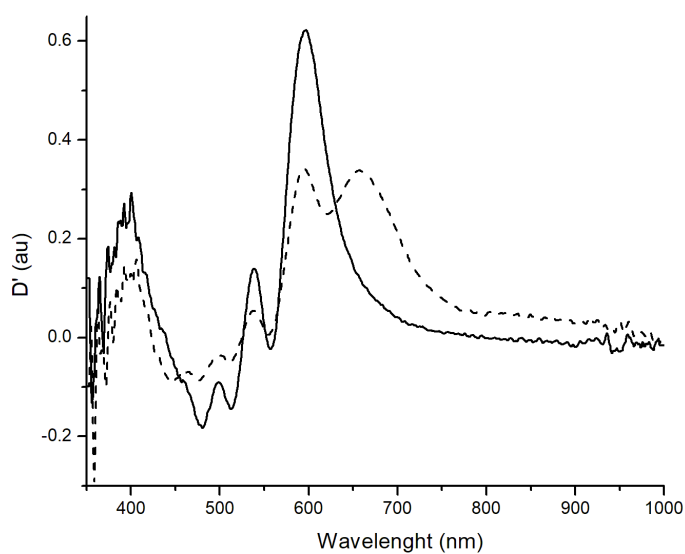
Figure 3: First derivative spectra of animal red dyes: cochineal (solid line) and lac (dash line), both etched with alum.
