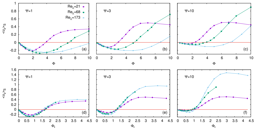
FIGURE 3. Average of the vertical fluid velocity, \langle u_z \rangle_S , along swimmer trajectories for rod-like ( \alpha = 1 ) cells as a function of \Phi = v_s/u_\eta (panels (a), (b) and (c)), and of \Phi_L = v_s/u_{\text{rms}} (panels (d), (e) and (f)) for different Re_\lambda , as labeled in (a). While the small \Phi behavior in the top panels rescales consistently, the transition to preferential sampling of positive values of u_z is better rescaled by \Phi_L .
