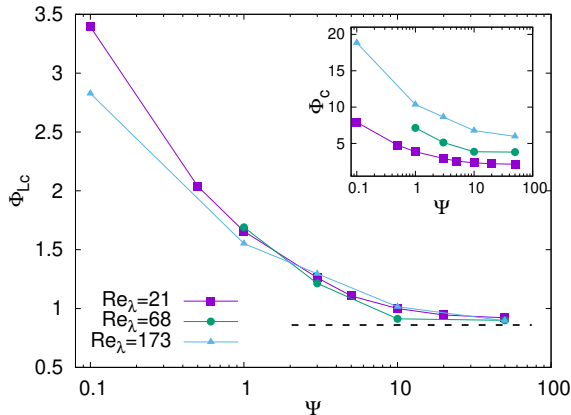
FIGURE 4. Critical value of \Phi_L (main panel) and \Phi (inset) for various \text{Re}_\lambda as a function of \Psi . Dashed line: theoretical asymptotic value of \Phi_{L,c} (see text).
