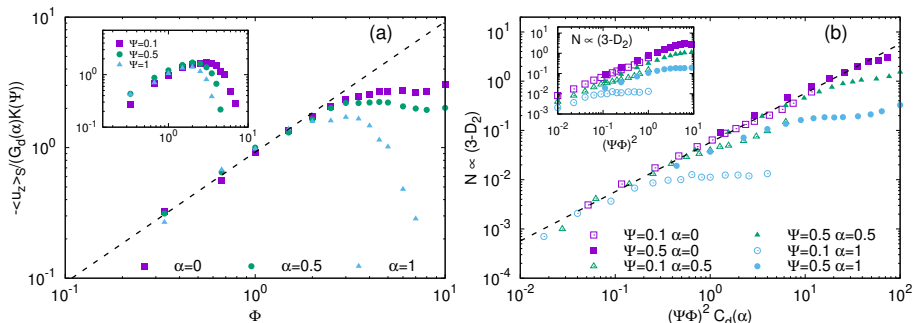
FIGURE 2. Small \Phi behavior of preferential sampling of fluid velocities and small scale clustering, compared with the theoretical predictions in Gustavsson et al. (2016) (dashed lines). a) vertical component of fluid velocity conditioned on swimmer trajectories for different elongations \alpha as labeled at \Psi = 0.1 . Inset: same as main panel but for rods ( \alpha = 1 ) at different \Psi . b) Accumulation index N rescaled with the stochastic prediction. Inset: the same curves without rescaling.
