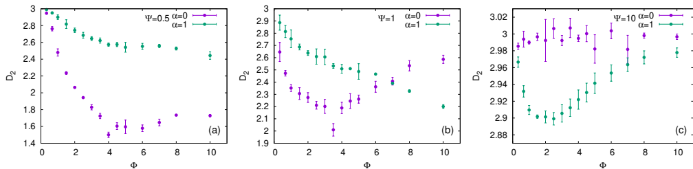
FIGURE 5. Correlation dimension of clusters for \Psi = 0.5 (a), 1.0 (b) and 10 (c) as a function of the swimming parameter \Phi . Spherical swimmers ( \alpha = 0 ) concentrate more than elongated cells (in this case, ideal rods) for small values of \Psi (a), while rod-like swimmers maintain observable clustering even for large \Psi (c). For intermediate values of \Psi , slow (fast) elongated swimmers cluster less (more) than spherical ones (b).
