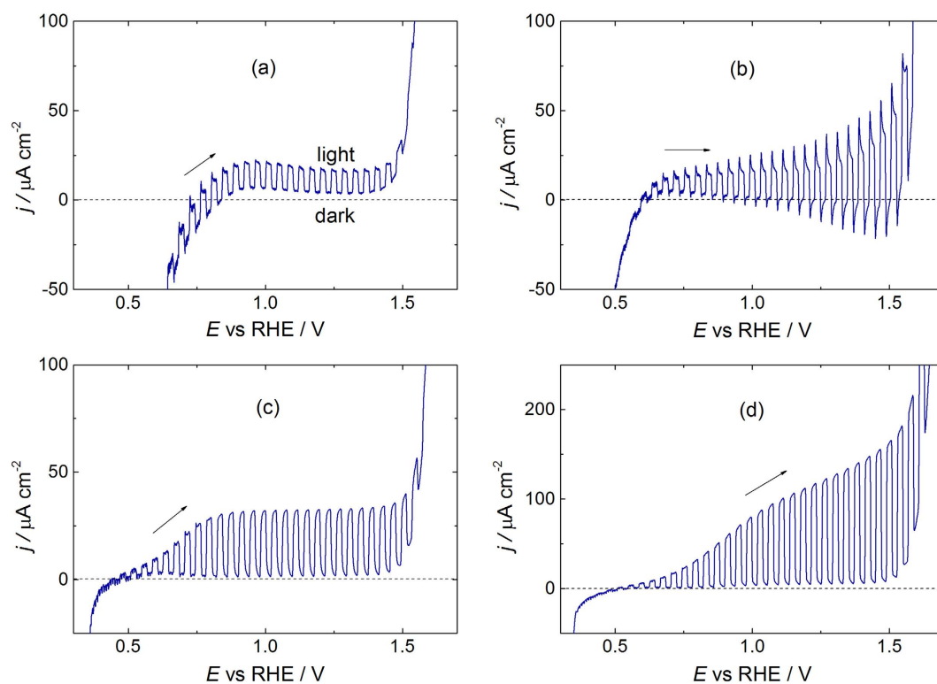
Figure 5. Voltammograms (scan rate 20 mV s -1 ) under chopped white light (Xe lamp, power \cong 1 sun). (Top): 1 M NaOH, electrodes: (a) FTO/Hematite-NRs; (b) FTO/hematite-BL/hematite-NRs. (Bottom): 0.1 M NaOH + 0.2 M LiI, electrodes: (c) FTO/Hematite-NRs; (d) FTO/Hematite-BL/Hematite-NRs.
