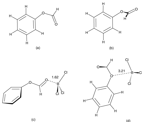
Scheme 5. Structures of phenyl formate and its complexes with BCl 3 (B3LYP/6-31G(d,p) geometry). In (a) and (b) two stable conformers of phenyl formate are represented, whereas (c) and (d) depict the structure of the O-acyl and O-aryl adducts, respectively.
