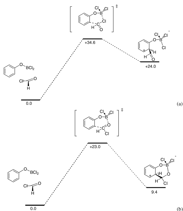
Fig. 7. Potential energy surface for path (b1). (a) \text{B}\cdots\text{Cl} assisted; (b) \text{B}\cdots\text{O} assisted.
