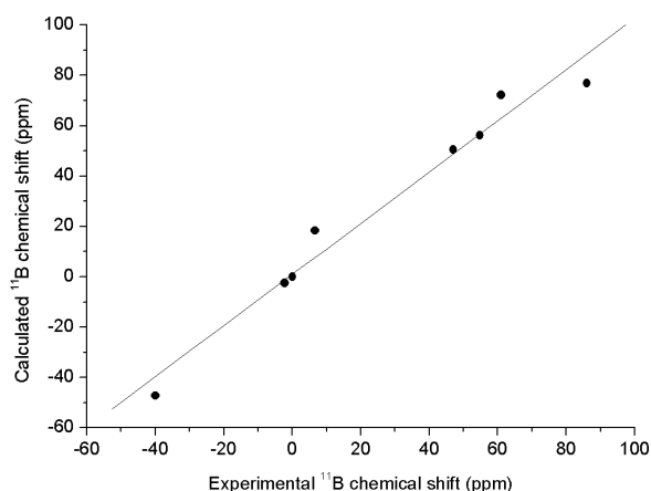
Fig. 1. Correlation between experimental and calculated 11 B chemical shifts (data from Table 1). Bromine-containing compounds are excluded since they show major deviations from the correlation (see text). The linear regression has slope 1.01, intercept 0.95 ppm, r = 0.97 .
