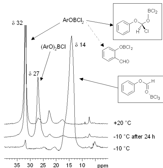
Fig. 2. ^{11}\text{B} NMR Spectra of the phenyl formate- \text{BCl}_3 mixture. Lower trace: After mixing at -10^\circ\text{C} ; middle trace: after 24 h at -10^\circ\text{C} ; upper trace: after thawing at 20^\circ\text{C} .
