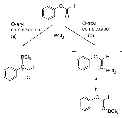
Scheme 2. Possible complexation modes of phenyl formate with boron trichloride.
