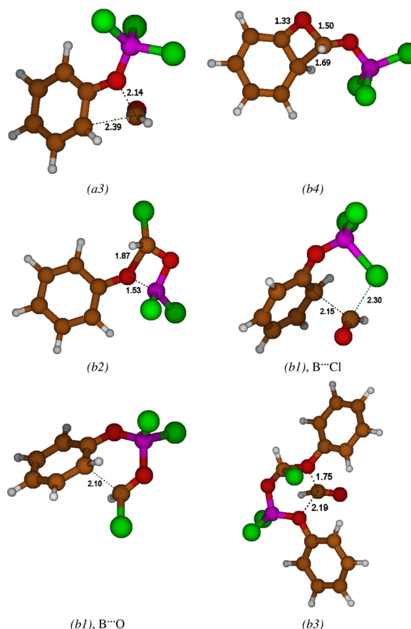
Fig. 9. Calculated structures of the transition states for all mechanisms investigated. Some relevant interatomic distances are given in Å.
