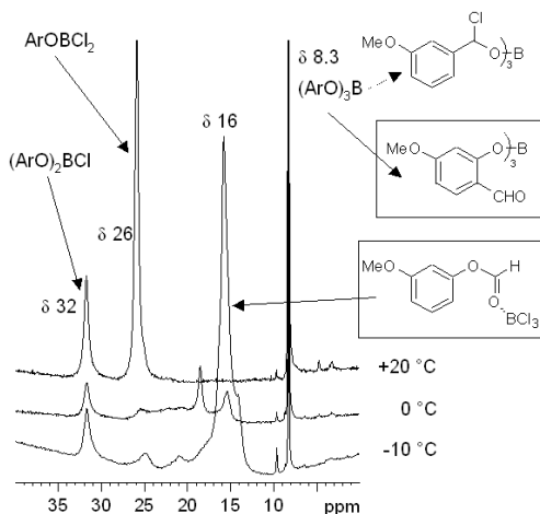
Fig. 3. ^{11}\text{B} NMR Spectra of the 3-methoxyphenyl formate- \text{BCl}_3 mixture. Lower trace: After mixing at -10^\circ\text{C} ; middle trace: 0^\circ\text{C} ; upper trace: after thawing at 20^\circ\text{C} .
