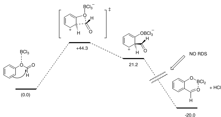
Fig. 4. Potential energy surface for the intramolecular Friedel-Crafts acylation from the O -aryl complex, path ( a3 ). The step marked as “NO RDS” is assumed to be not rate-determining.
