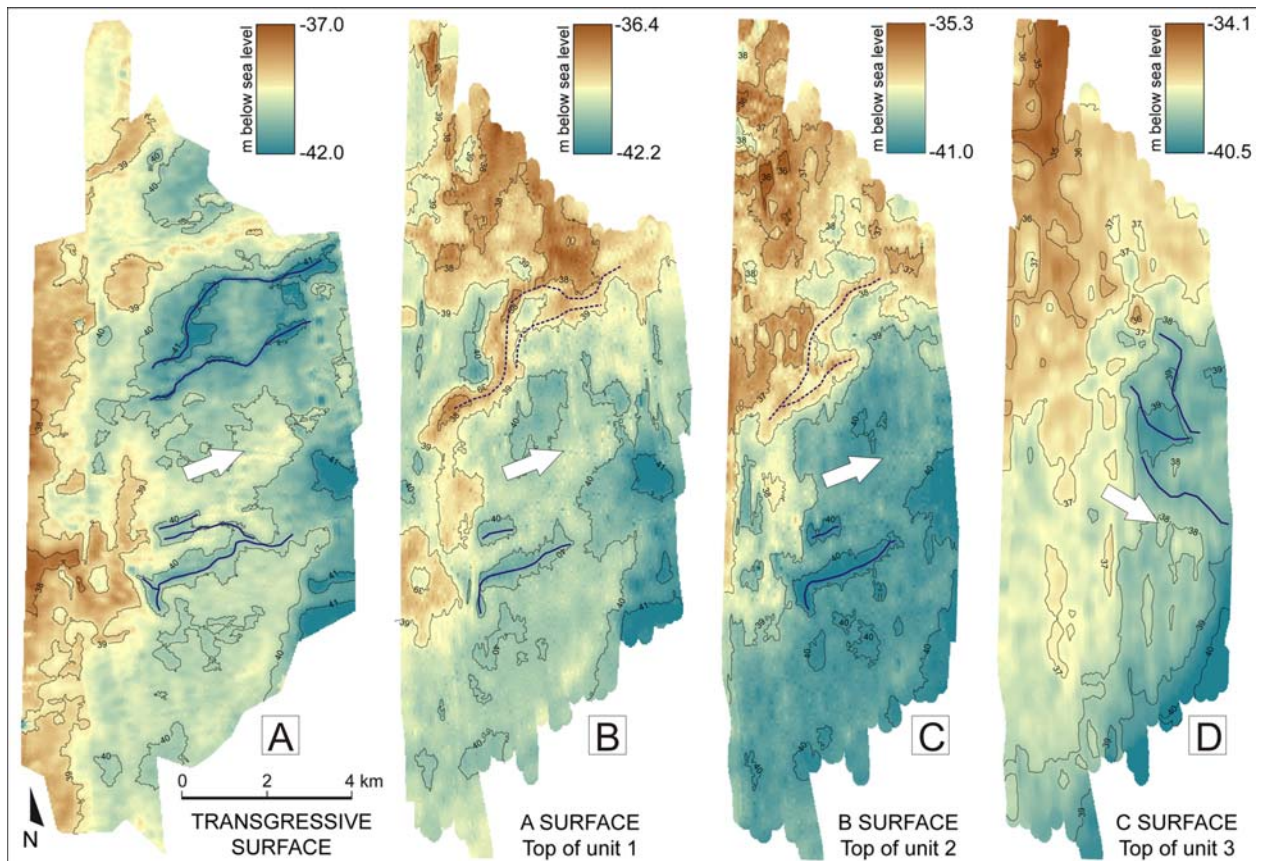
Fig. 6 - DEMs with isopach of the key surfaces obtained from Conversion Tools ASCII to Raster of ArcMap 10.1 program. Comparison of DEM. Variation in channel system trend and preservation of each unit. The channels depicted in each surface have been traced in blue, while the dashed rivers represent the leveed channel systems elevated above the underlying surface.
