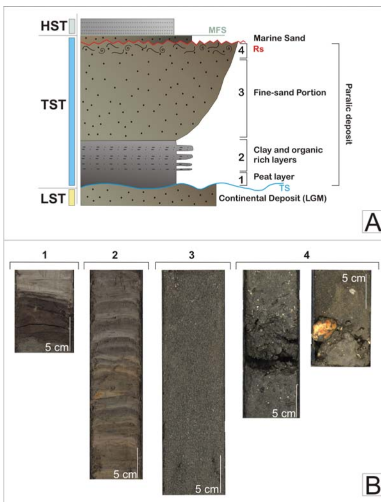
Fig. 3 - Main cores facies description. (A) Simplified log of most representative cores. The TST deposits rest on the Transgressive Surface. The paralic deposit is characterized at the base by clay sediment, peat and organic-rich layers and at the top by a sand portion. This deposit ends with ravinement surface. (B) Example of cores facies. 1: peat layer; 2: interbedded clayey and silty layers; 3: sand portion; 4: ravinement surface (Rs).
