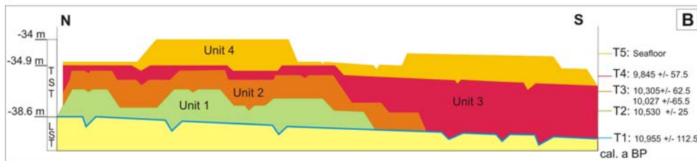
Fig. 8 - A: Depth vs. Age Plot. In blue are represented the Adriatic 14 C data from composite table in Antonioli et al. (2009) and from Geological Map of the Italian Sea (Fabbri et al., 2001; Trincardi et al., 2011 a-b). In orange are represented the Radiocarbon dating from this work. In grey are represented Th/U data from Fairbanks (1992) and Bard (2003). B: Simplified scheme of the transgressive deposit with water depth and age of each unit.
