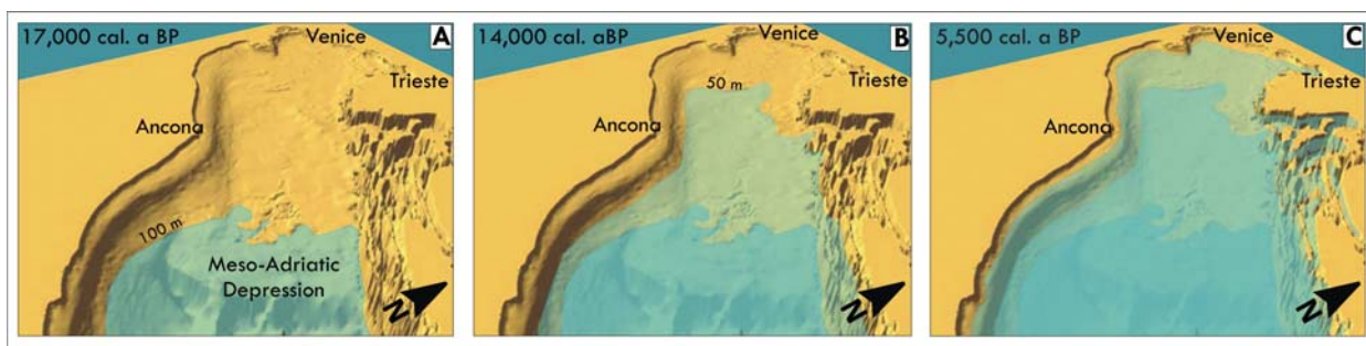
Fig. 2 - Widening of the Adriatic basin during the last transgressive cycle. (A) Sea-level during the Last Glacial Maximum (LGM), an extensive portion of the Adriatic sea was in subaerial condition, while the Meso-Adriatic-Depression (MAD) was a semi-enclosed basin receiving high amount of sediment (Correggiari et al., 1996). (B) Rapid sea-level rising after the LGM. (C) Maximum marine ingression reached 5500 cal. a BP.
