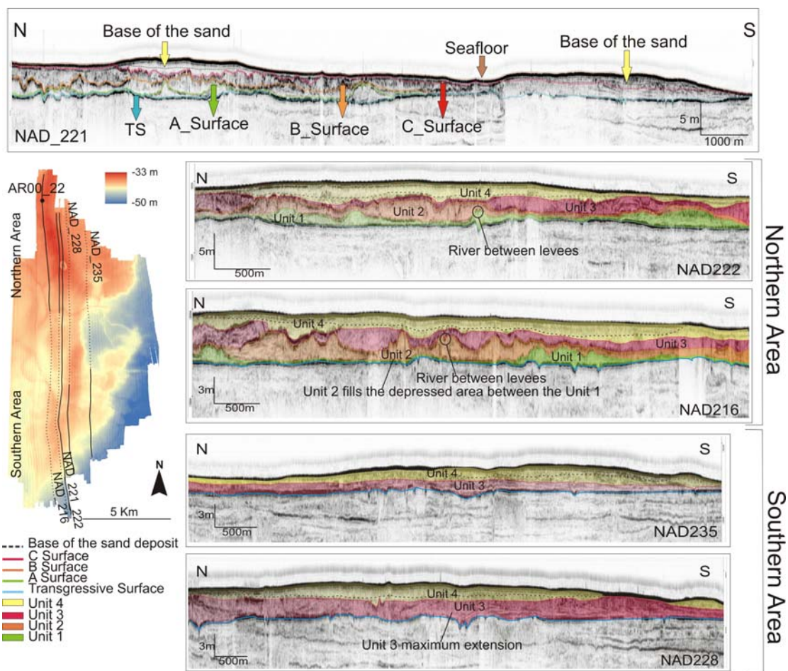
Fig. 5 - Evidence of the key surfaces and units within the sedimentary transgressive body.
