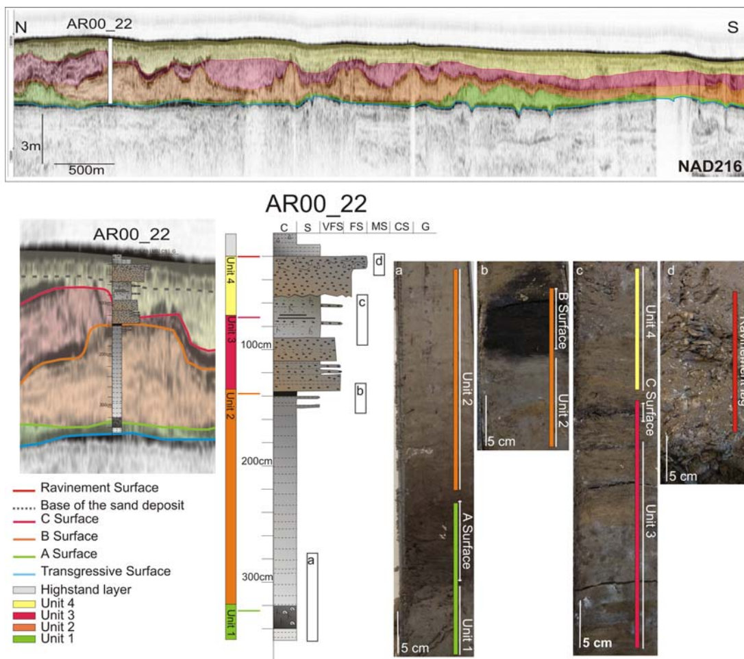
Fig. 7 - AR00_22 core log plotted on NAD216 seismic profile, location in Fig. 5 . On the left, the picture shows the position of AR00_22 in the seismic profile, the seismic units in color bordered by the key surfaces. On the right, the picture shows the description of the AR00_22 core, their core facies, highlighted by the photos, corresponding to the white panels a, b, c, d close to the core log.
