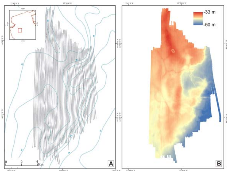
Fig. 4 - Study Area detail. (A) Tracks of VHR seismic profiles, acquired in 2012, covering the study area. (B) Seafloor bathymetry (image resolution of 10 m). Evidence of the ESE channel system trend.
