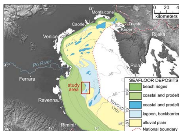
Fig. 1 - Location of the study area in the Adriatic Sea. Bathymetry and superficial geology modified from the Geological Map of Italian seafloor (Fabbri et al., 2001; Trincardi et al., 2011 a, Trincardi et al., 2011 b).
