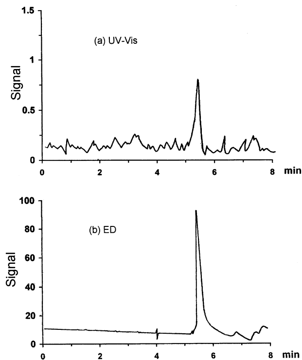
Fig. 5. Comparison between the UV-vis (a) and the ED (b) response of (8). Mobile phase: acetonitrile containing LiClO_4 (0.01 M), room temperature; flow rate: 0.7 \text{ ml min}^{-1} .
