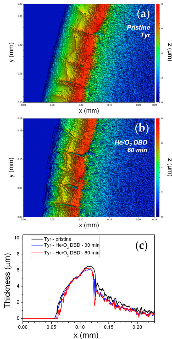
Figure 4. 2D white light vertical scanning interferometry (WLVI) images of a 5 \mu\text{g} Tyr deposit (a) before and (b) after exposure to a He/1% O 2 fed DBD for 60 min ( f = 20 kHz, V_a = 1.1 kV rms ). (c) Cross-section thickness profiles of the Tyr deposit before and after exposure to the He/1% O 2 fed DBD for 30 and 60 min.
