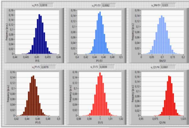
Fig. 8. Monte Carlo results in the case of all nonlinear loads (original configuration). Load L2.
