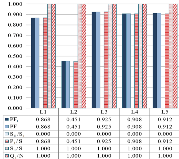
Fig. 5. Simulation results of the power ratios in the case of all linear loads. Power ratios from the arithmetic approach.
