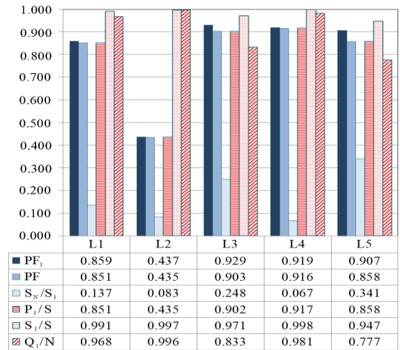
Fig. 6. Simulation results of the proposed approach in the case of all nonlinear loads (original configuration). Power ratios from the arithmetic approach.
