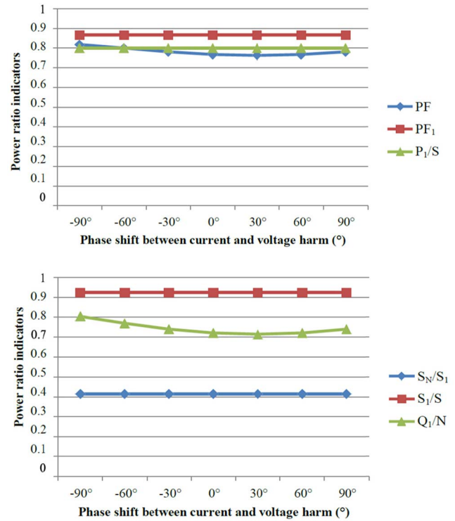
Fig. 3. Results of indicators. Experimental test with the fifth harmonic on both voltage and current; 30^\circ phase shift between both fundamental and harmonic components; and phase shift between harmonic components from -90^\circ to +90^\circ .
