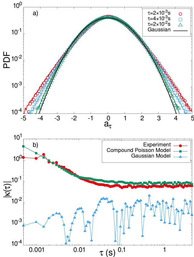
FIG. 3. Statistical distribution of the standardized angular velocity increments a_\tau(t) = \Delta_\tau \omega / \sqrt{\langle (\Delta_\tau \omega)^2 \rangle} : comparison between models and the experiment with N = 1000 . In panel a) we show the distributions of the variables at three different lag-times \tau : the empty symbols are experimental data, while solid curves are the interpolation of the numerical integration of the model in Eq. (1) with Poisson compound noise \xi_1 . The black line is the normal distribution for reference. Panel b) shows the absolute value of the excess kurtosis \kappa(\tau) as a function of \tau for experimental measurements (red circles) and numerical simulations with \xi_1 chosen to be a compound Poisson noise (green squares) or white noise (blue triangles).
