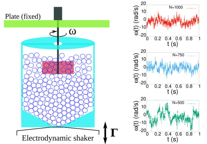
FIG. 1. Scheme of the experimental setup (left) and time series of the probe's angular velocity \omega(t) (right) for different values of the number of spheres N .
