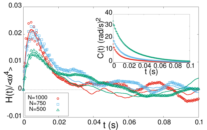
FIG. 4. Comparison between experiments with different N . The empty symbols are experimental data, while solid curves come from numerical integration of the model in Eq. (1) with Poisson process for \xi_1(t) . The inset shows the corresponding correlation functions.
