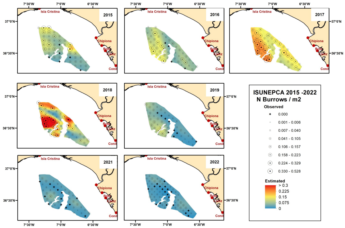
Fig. 1: Map of density by station for each year. Data updated after re-definition of the UVTV survey area. Bubble plot of the burrow density observations overlaid on a krigged burrow density surface for UWTV survey series (2015-2022; 2020 not available due COVID-19 pandemic). Station positions with zero density are indicated using a +.
