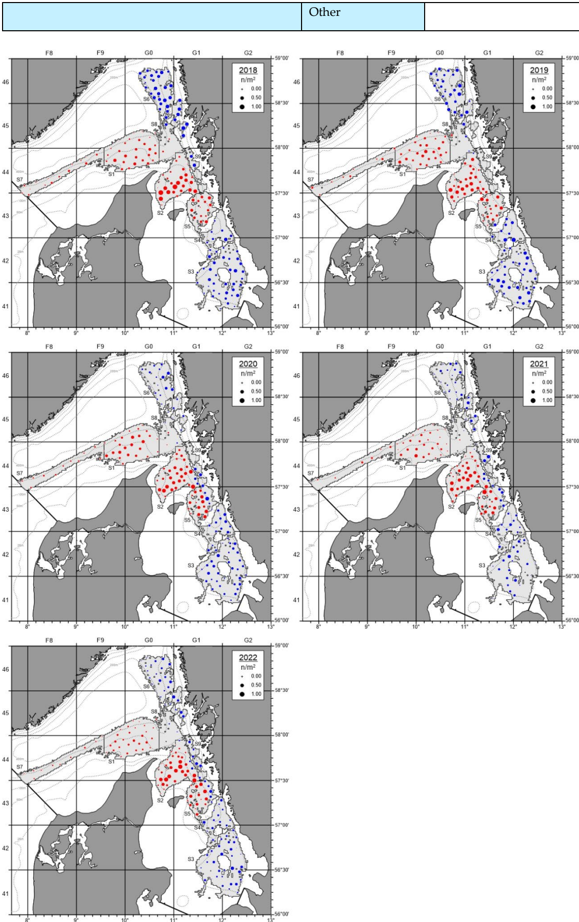
Fig. 1b: FU 3&4 (Skagerrak/Kattegat) Nephrops burrow density by station 2018 - 2022 (red: DK, blue: SWE).
