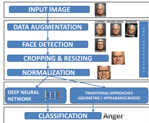
Fig.1. Pipeline of the proposed system. First a pre-processing task on the input images was performed. The obtained normalized face image is used to train the deep neural network architectures. Moreover, both geometrical and appearance-based features are extracted from normalized image. Finally, each image is classified by associating it with a label of most probably facial expression.
