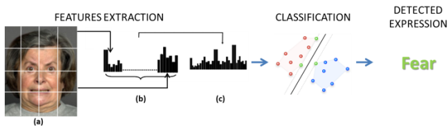
Fig.6. Appearance-based approach used for FER in ageing adults: (a) facial image is divided into non-overlapping blocks of 8x8 pixels, (b) for each block the LBP histogram is computed and then concatenated into a single vector (c). The classification module is based on an SVM classifier able to output the most probable expression
