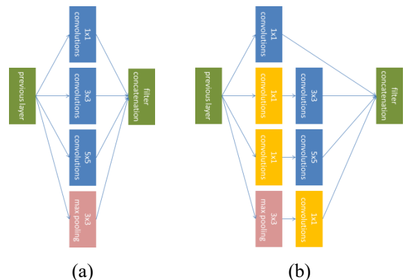
Fig.4. (a) Schematic representation of Inception module architecture (original version). (b) Schematic representa-
