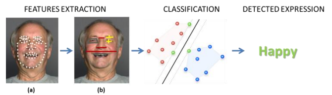
Fig.5. FER based on the geometric features extraction methodology: (a) facial landmark localization, (b) extraction of 32 geometric features (linear, elliptical and polygonal) using the obtained landmarks. The classification module is based on an SVM classifier able to output the most probable expression.
