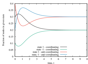
FIGURE 5. Evolution over time of the fraction of nodes in the ABRD game, according to analysis.
