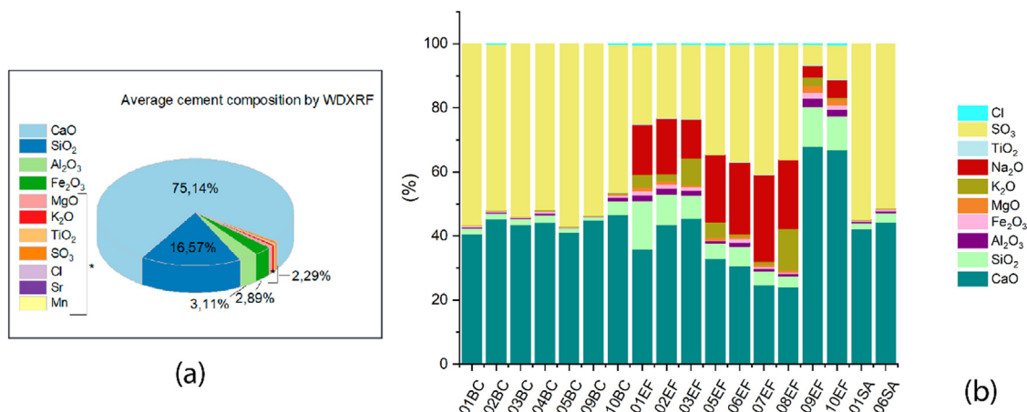
Fig. 4. (a) Average cement composition determined by WDXRF. (b) Elemental distribution determined by WDXRF for samples under study. The samples of black and white crusts present the highest percentages of sulphur, while the efflorescence samples have the highest percentages in sodium and chlorine.
