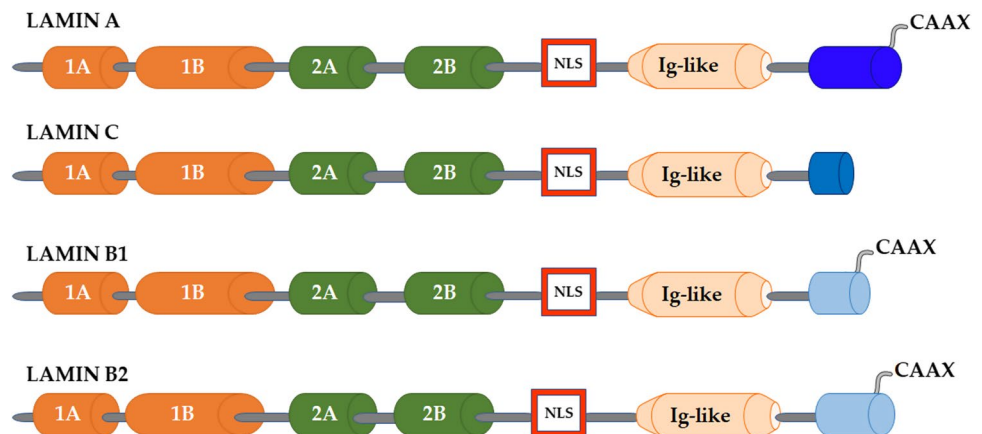
Fig. 1 Domain organization of the main human lamin isoforms. The α-helical rod domain comprises four segments, 1A, 1B, 2A, 2B, which are separated by linker segments. The C-terminal tail domain contains a nuclear localization signal (NLS), an immunoglobulin domain (Ig-like), and a conserved CAAX box, which undergoes farnesylation
