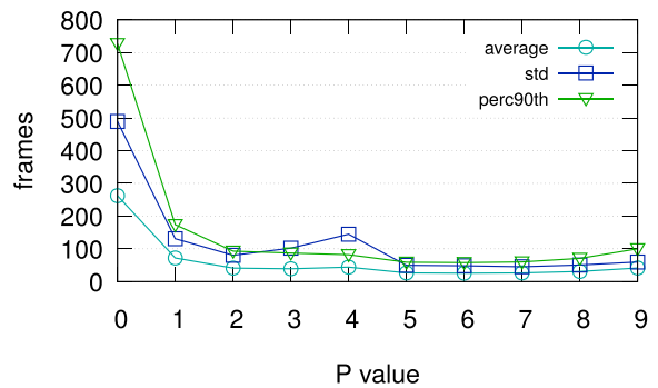
(b) Descriptive statistics of \Theta length
