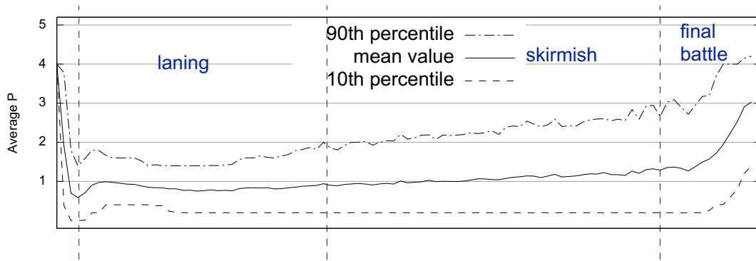
Fig. 4 Average AoI population over time
