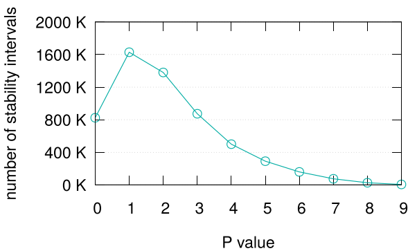
(a) Frequency of \Theta s as a function of P
