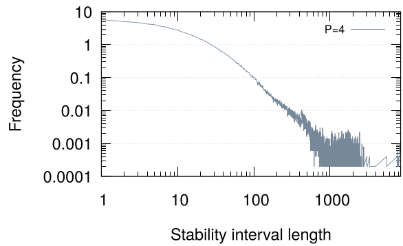
(d) Log-log plot of \Theta lengths with P = 4
