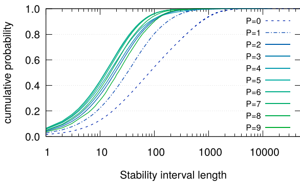
(c) Log-scale CDF of \Theta length for all P
