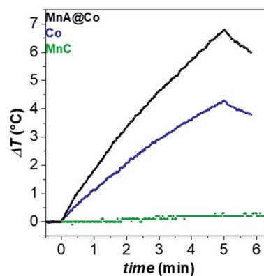
Fig. 7 Heating curves of aqueous colloidal dispersions of samples ( C_{ox} = 3.4 \text{ mg mL}^{-1} ) at 30 °C. The magnetic field was 183 kHz and 17 kA m^{-1} .
