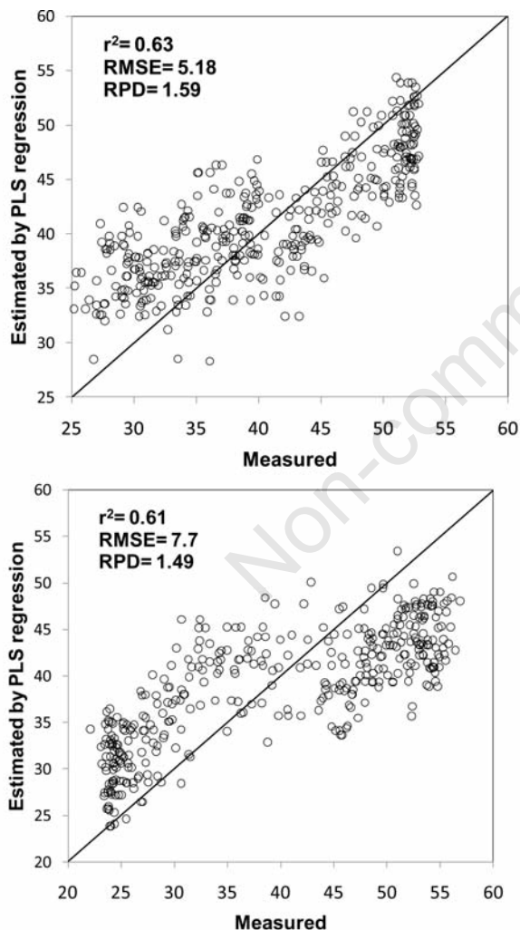
Figure 2. Measured vs estimated clay (top) and sand (bottom) values resulting from the application of PLSR to the validation set for field B071 using spectral reflectance data extracted from the CHRIS-PROBA image.
