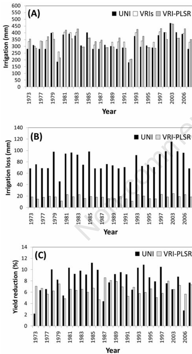
Figure 5. Simulation results for the comparison of irrigation strategies for field B071. A) total seasonal irrigation. B) irrigation losses due to percolation. C) reduction from the potential yield.
