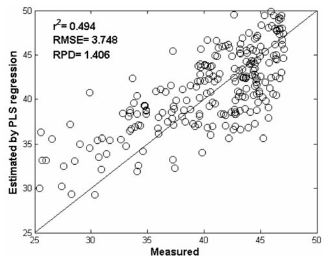
Figure 1. Measured vs estimated clay values resulting from the application of PLSR to the validation set for field B064 using spectral reflectance data extracted from the CHRIS- PROBA image.
