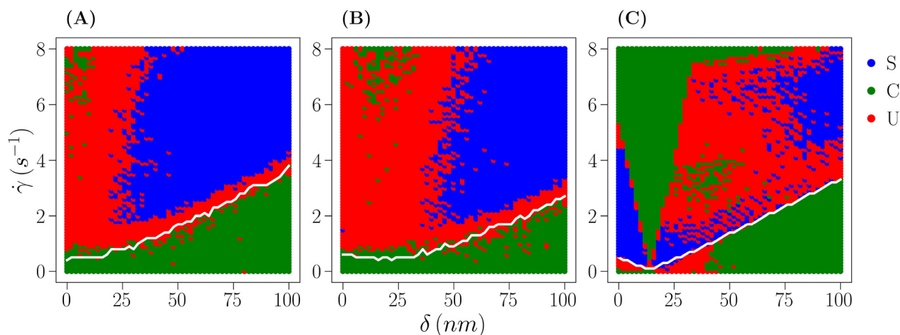
Fig. 6 State diagram of a bottom-heavy Janus particle under varying shear flow ( \dot{\gamma} = 0-8 \text{ s}^{-1} ) and cap thickness ( \delta = 0-100 \text{ nm} ) for: (A) R = 1 \mu\text{m} , \psi_1 = -20 \text{ mV} , \psi_2 = -20 \text{ mV} and \psi_w = -50 \text{ mV} . (B) Same as in (A), but \psi_2 = -40 \text{ mV} . (C) Same as in (B), but R = 4 \mu\text{m} . The white line is the same transition line drawn in Fig. 4, and colors represent the classification of each state point as described by the legend on the right. Symbols in the legend stand for sinusoidal (S), i.e. , non-constant angular velocity, constant (C), i.e. , constant angular velocity, and unclassified (U).
