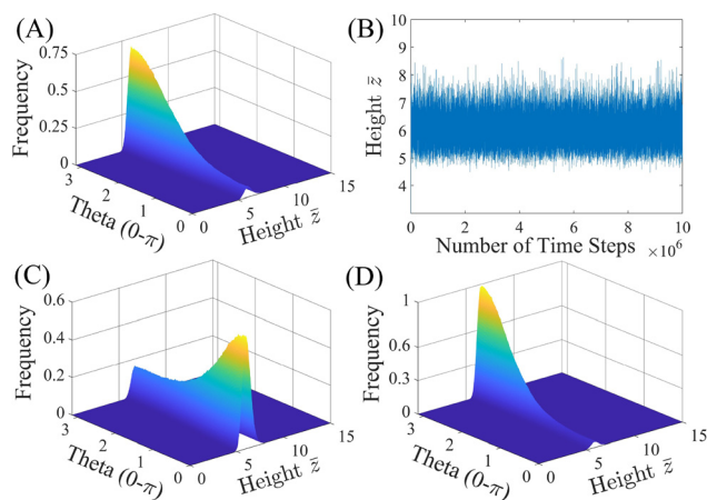
Fig. 3 Impact of cap thickness and surface potential on the probability density function (PDF) of a bottom-heavy Pt-capped Janus particle of R = 1 \mu\text{m} with cap thickness, \delta , and surface potentials, \psi_1 and \psi_2 , interacting with a wall of surface potential, \psi_w = -50 \text{ mV} using model II: (A) PDF and (B) equilibrium height \bar{z} for \psi_1 = \psi_2 = -20 \text{ mV} and \delta = 10 \text{ nm} . (C) Same as (A) with \psi_2 = -40 \text{ mV} . (D) Same as (C) with \delta = 30 \text{ nm} .
