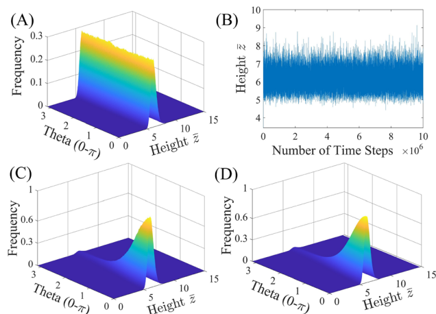
Fig. 2 Impact of surface potential, \psi , on the probability density function (PDF) for a Janus particle of R = 1 \mu\text{m} without a cap ( \delta = 0 ), with surface potentials, \psi_1 and \psi_2 , interacting with a wall of surface potential, \psi_w = -50 \text{ mV} , using model 0: (A) PDF and (B) equilibrium height for \psi_1 = \psi_2 = -20 \text{ mV} and model I: (C) PDF for \psi_1 = -20 \text{ mV} and \psi_2 = -40 \text{ mV} . (D) Boltzmann distribution prediction of the orientation distribution for the particle simulated in (C).
