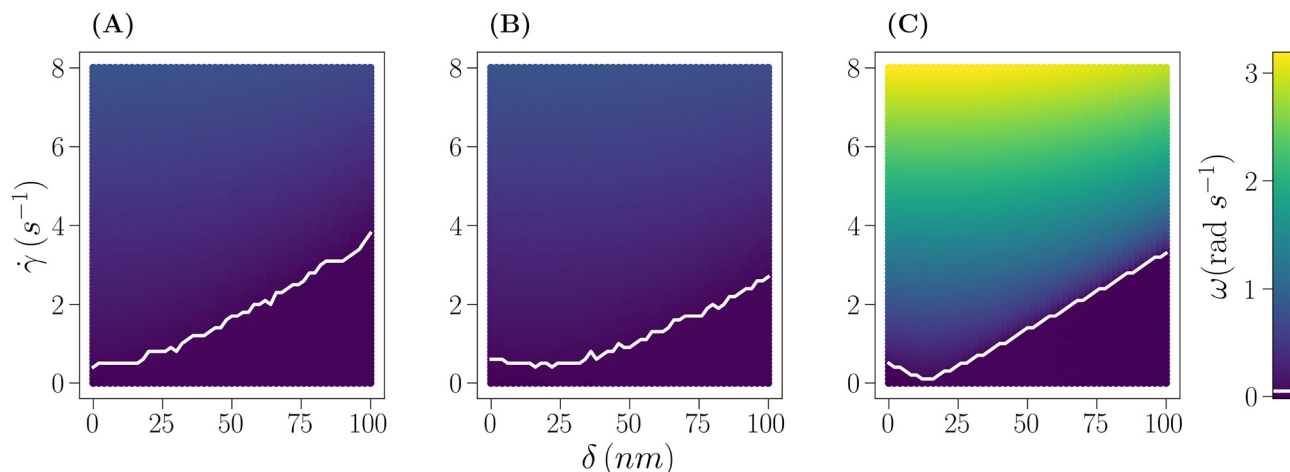
Fig. 4 Angular velocity maps for a bottom-heavy Janus particle under varying shear flow ( \dot{\gamma} = 0-8 \text{ s}^{-1} ) and cap thickness ( \delta = 0-100 \text{ nm} ) using model III for: (A) R = 1 \mu\text{m} , \psi_1 = -20 \text{ mV} , \psi_2 = -20 \text{ mV} and \psi_w = -50 \text{ mV} . (B) As in (A), but \psi_2 = -40 \text{ mV} . (C) As in (B), but R = 4 \mu\text{m} . The color represents the average angular velocity as displayed by the color bar on the right. The transition line (white) is drawn at \omega = 0.05 \text{ s}^{-1} .
